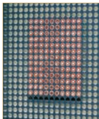
Details of transfer using Optical Beam Waveguides
