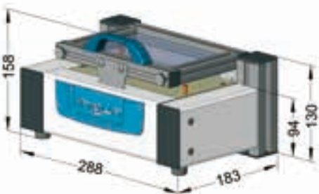
Detailed dimensional drawing of: MA 160 with ATS 160
