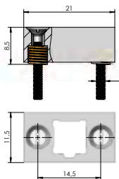
HAS-819/ HAS-819 160 (Consisting of Contact Mounting, Threaded Pins, Springs and Screws)
