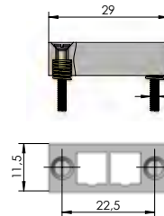
HAS-819 D8-160 (Consisting of Contact Mounting, Threaded Pins, Springs and Screws)
