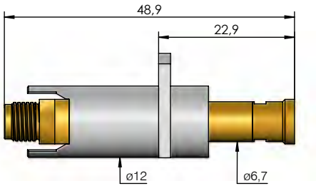
Connection for Screw-in Plug SE-819-V5-Z
