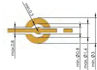
PCB coax kidney-shaped
