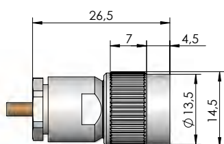
PC3.5-m (straight)
