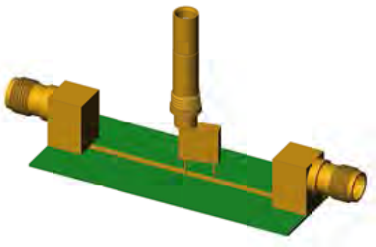
Example of test set-up with three-port measurement
