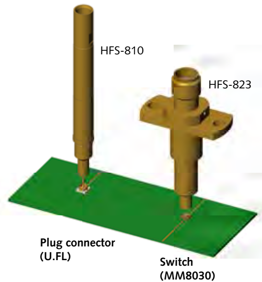
Example of plug connectors from communication and consumer electronics
