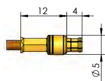
MCX-plug (straight)*
