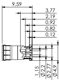
Signal Conductor Plug
