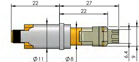
Connection for USB-Mini Plug
