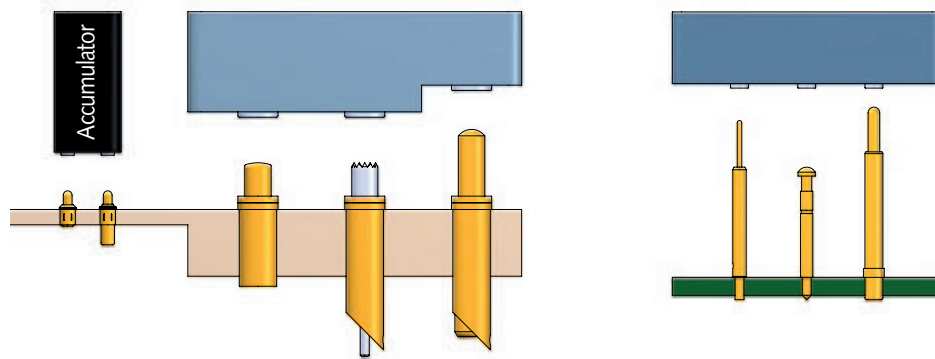
Test probe as contact element
